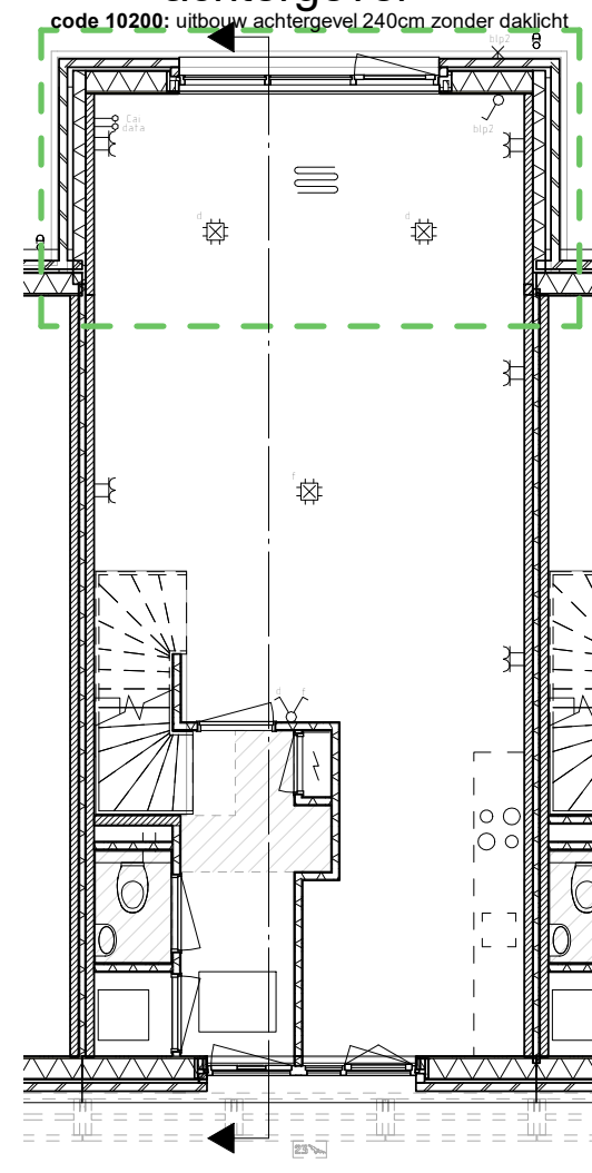
00 begane grond
